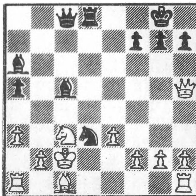
219 After 18 Qh5
